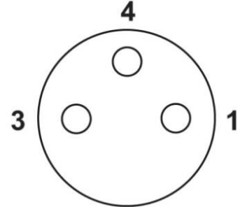
Pin assignment M18-jack, 3-pol, A-coding
